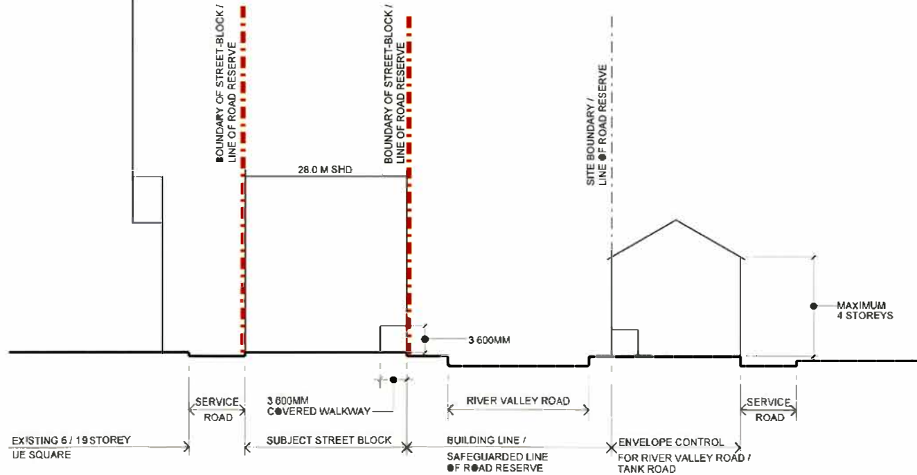
TYPICAL SECTION OF STREET BLOCK SCALE : 1 : 500
