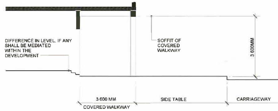
COVERED WALKWAY DETAILS SCALE : 1 : 100
